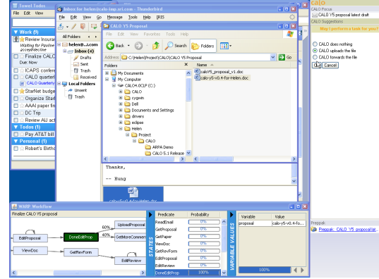
Figure 2: Context-aware assistance provided by PEXa.
