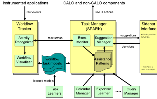
Figure 1: Partial architecture of the PEXa agent.
