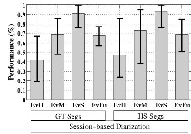
Figure 4. Average, lowest, and highest performance results for each experimental condition and evaluation strategy.
