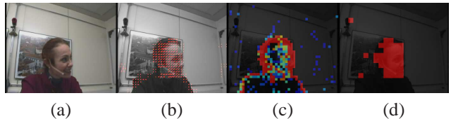
Figure 2. Compressed domain video feature extraction. (a) Original image, (b) Motion vectors, (c) Residual coding bit-rate, (d) skin-coloured regions.
