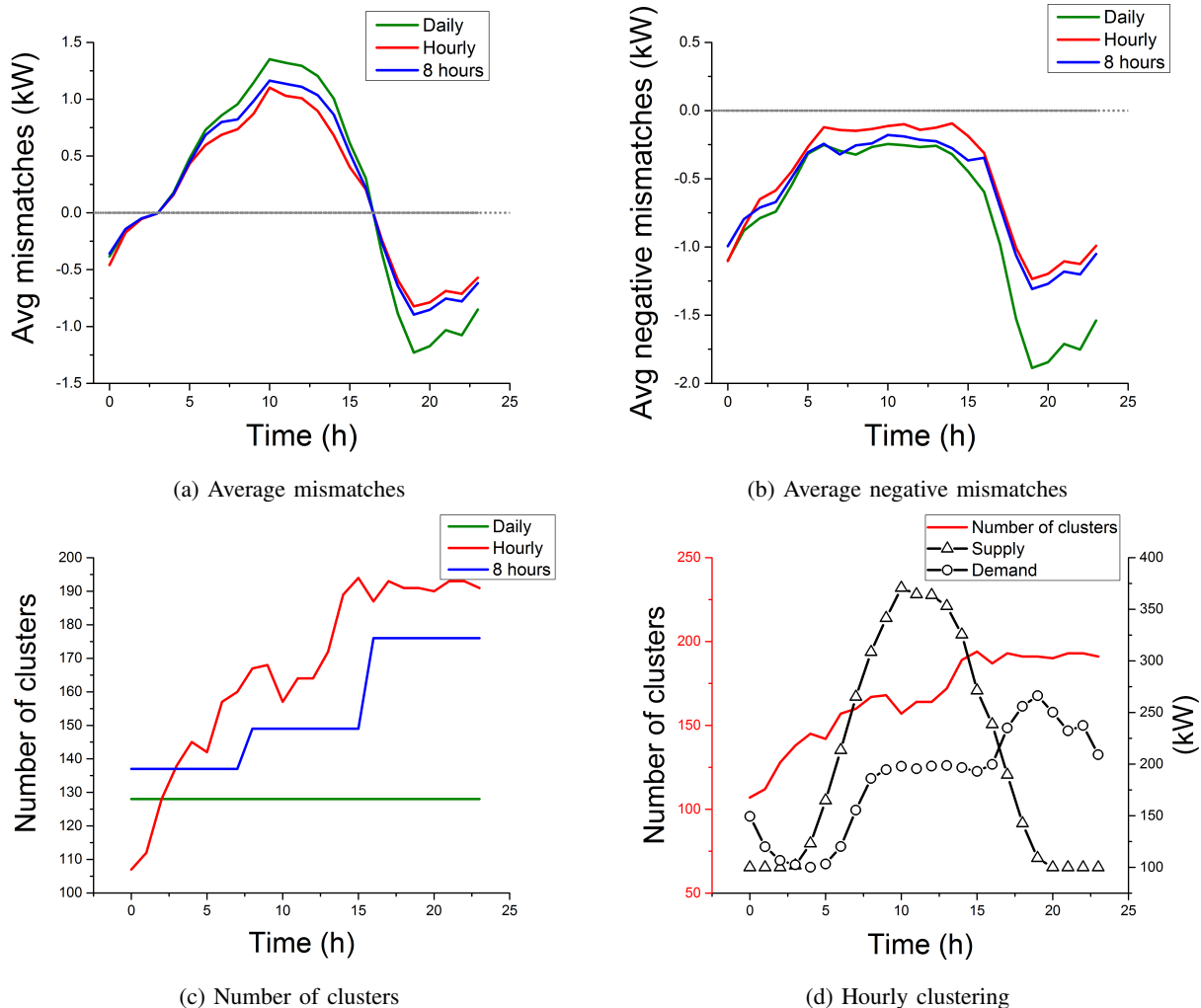
Fig. 2: A comparison of static (daily) and dynamic (every 8 hours and hourly) clustering (based on 100 algorithm runs)
