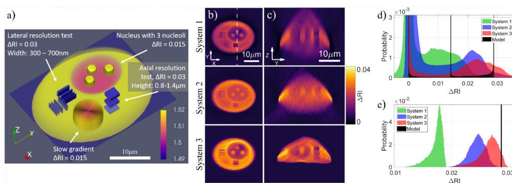
Figure 11. (a) CAD model of the 3D cell phantom. (b,c) Cross-sections of the 3D RI distribution of the phantom measured using three different holographic tomographs with a limited angle of projections. (d,e) Histograms of the \Delta RI in case of full measurement volume (d) and manually segmented single nucleoli (e).
