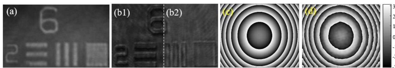
Figure 6. (a,b2) Reconstructions of thin ( OT < \lambda ) phase-only object by the iterative approach when initialized with regular intensity measurement (b1) and phase-contrast measurement (not shown), respectively (Adapted from [73]). (c) Theoretical and (d) reconstructed phase of a refractive lens ( OT > \lambda ) by using the phase-shifting method (Adapted from [71]).
