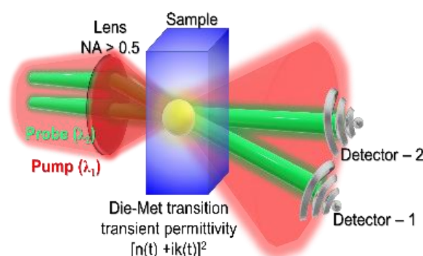
Figure 7. The pump ( \lambda_1 ) two-probes ( \lambda_2 ) method allows the recovery of permittivity transient, separation of the phase delay, and absorbance contributions at the wavelength of probe ( \lambda_2 ). Light-matter interaction from the focal region is fully defined by the instantaneous permittivity (square of the complex refractive index [n(t) + ik(t)]^2 ). The configuration can be applied to both transmission and reflection modes.
