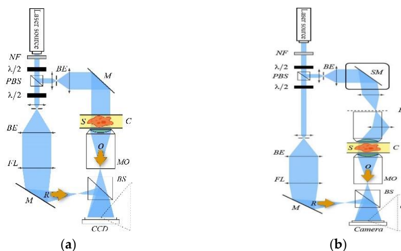
Figure 1. (a) example of optical setup for transmission Digital Holographic Microscopy DHM. (b) Optical setup for Tomographic Diffractive Microscopy: Laser source with controllable coherence length. NF neutral filter, \lambda/2 plate, PBS polarizing beam splitter, BS beam splitter, BE beam expander, SM steering mirror and M mirror, BF back focal plane, S specimen, C cell, O object wave, R reference wave.
