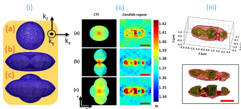
Figure 9. (i): Comparison of coherent transfer functions (CTF) of (a) BR, (b) SR, and (c) IDT. (ii): Comparison of slices of 3D refractive index distribution of candida rugosa and the experimentally obtained CTFs corresponds to (a) SR approach, (b) BR approach, and (c) IDT approach. (iii): 3D illustration of candida rugosa at sub-cellular structural views; the different colors represent the different organelles of the cell. Scale bars: 2 \mu\text{m} . Adapted from [130].
