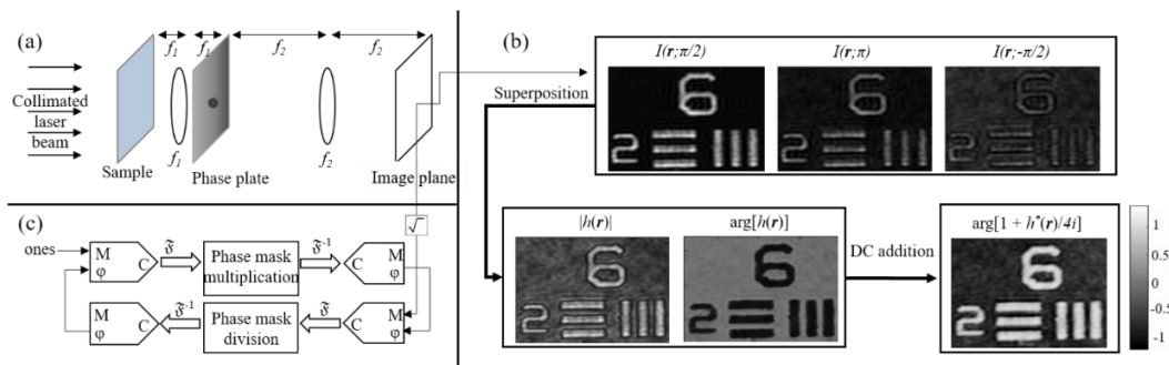
Figure 5. (a) Schematic of the self-reference on-axis apparatus used for QPI. (b) Flowchart of the phase-shifting process (Adapted from [71]). (c) Iterative QPI approach described in the text (Adapted from [73]).
