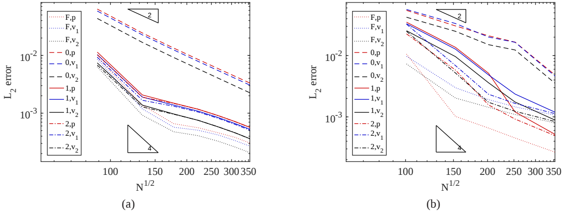
Figure 3 Convergence on a structured (a) and unstructured (b) mesh with the consistent mass matrix (dotted line), lumped mass matrix (dashes), 1 iteration (drawn) or 2 (dash-dotted line). Although the formal fourth-order accuracy is not obtained, the accuracy improvement with just one iteration compared to the second-order mass-lumped scheme is substantial.
