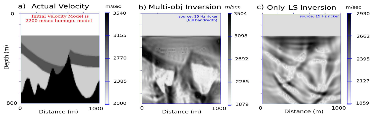
Figure 4: Fault model inversion results using a 15-Hz Ricker source. a) Actual velocity model used to generate the synthetic data. b) Full bandwidth multi-objective inversion result. c) Conventional least-squares waveform inversion result.
