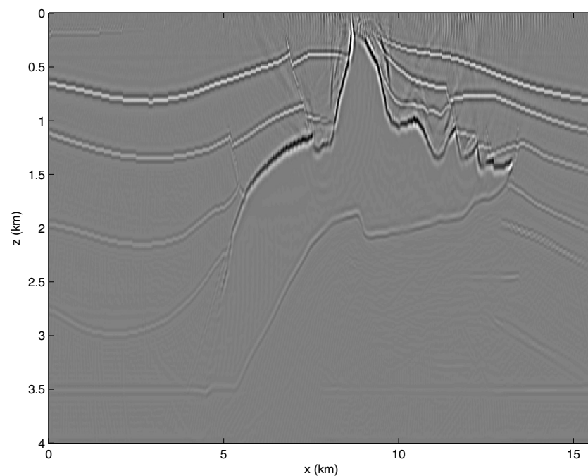
Figure 7. Migration result for the salt dome example without pre-conditioner.
