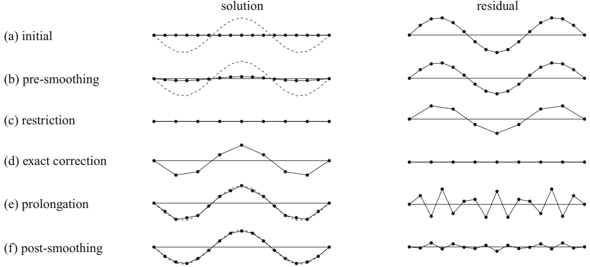
Numerical Methods, Multigrid, Fig. 1 Steps in a two-grid cycle. (a) The initial solution on the fine grid is set to zero and the residual equals the forcing function. The dash line represents the exact numerical solution. (b) After one step of pre-smoothing with damped Jacobi relaxation, the solution error is still large, and the residual has hardly changed in this example. Its restriction to the coarser grid (c) is solved exactly, using a coarse-grid version of the discrete differential operator.
