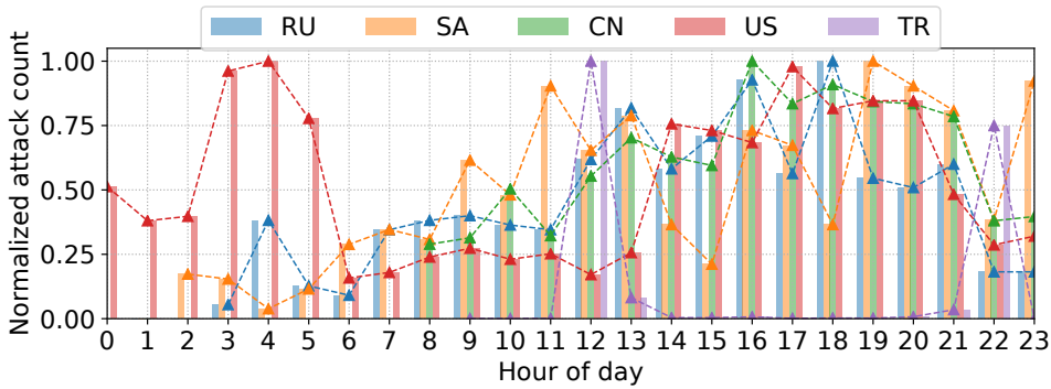
Figure 5.6: Local attack times for the top 5 victim countries. Attacks are mostly conducted in the afternoon and evening, except in the US where mainly data centers are targeted at night.
