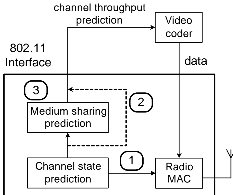
Figure 4.9: Cases of prediction. 1) – Channel state prediction. Used for Link Adaptation. 2) – Channel throughput prediction without considering medium sharing. 3) – Channel throughput prediction considering medium sharing.
