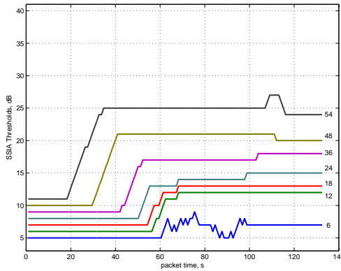
Figure 3.17: Adaptation of SSIA thresholds with low initial values.
