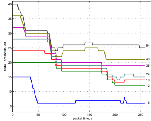
Figure 3.18: Adaptation of SSIA thresholds with high initial values.
