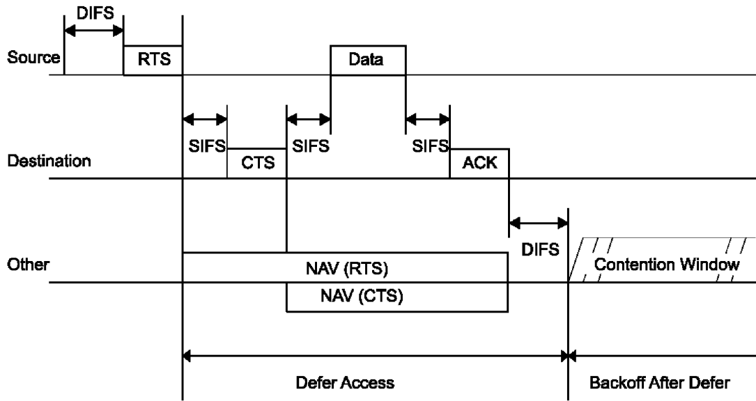
Figure 2.3: RTS-CTS mechanism
