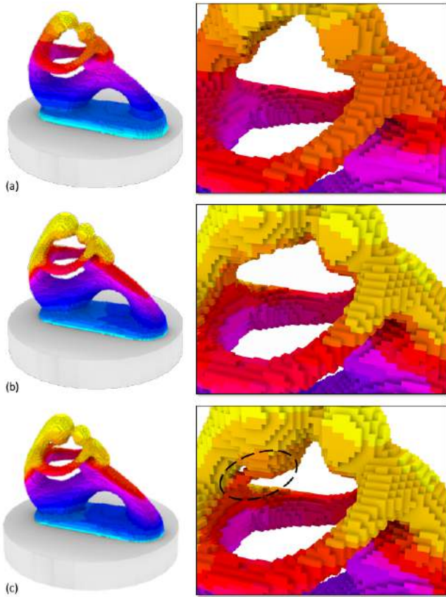
Fig. 14. An example of failure case – a Fertility model with 77, 064 voxels: (a) the result of SP-GCFA scheme (2,093 seconds with 1,376 voxels missed) and (b) the result of PG-SP-GCFA scheme (142 seconds – 14.7× faster but still have 511 voxels missed). After detecting the missed region and adding supports (encircled by dash line), the growing field can be successfully computed to cover the whole model (c) – PG-SP-GCFA scheme is used here (112 seconds).
