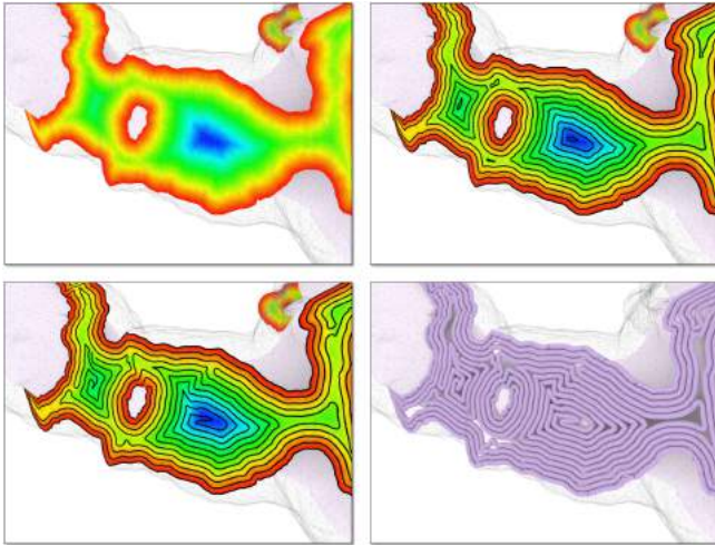
Fig. 8. An example for illustrating the generation of continuous Fernal spiral tool-path: (Top Row) The geodesic distance field is generated by the FWP-MMP method and the iso-contours are extracted on the mesh surface. (Bottom Row) The iso-contours at different iso-values are connected to form the tool-path.
