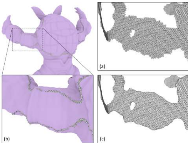
Fig. 7. An illustration for extracting a working surface with accurate boundary: (a) the isosurface S_i^* generated by dual contouring, (b) S_i^* is trimmed by \mathcal{H} , to obtain (c) the resultant working surface S_i with its boundary exactly located on the boundary of \mathcal{H} .
