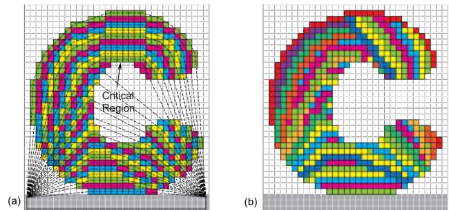
Fig. 6. An illustration of convex-front peeling and the peeling-governed convex-front advancing. (a) Isolated components will be generated when the voxels in the critical region are removed together with other voxels in the same layer. However, such problem on the peeling field F(\cdot) will be automatically avoided when shadow-region preserved convex-front advancing is conducted – see (b) for a result.
