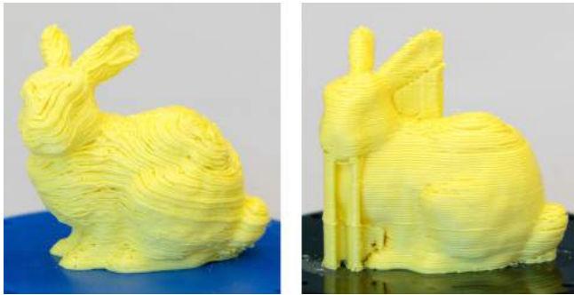
Fig. 16. A comparison for the Bunny model fabricated on the same robotic system by using different tool-paths: (left) the spatial tool-paths generated by our method and (right) the planar paths generated by conventional slicer for 3D printing.
