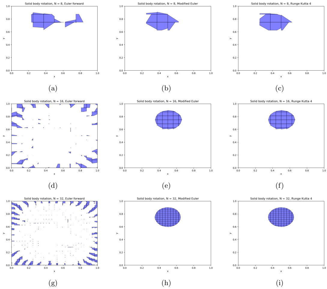
Figure 20: Volume of fluid fields for the test of table 1 using the solid body rotation velocity field. Higher order time stepping methods are required to make this test stable.
