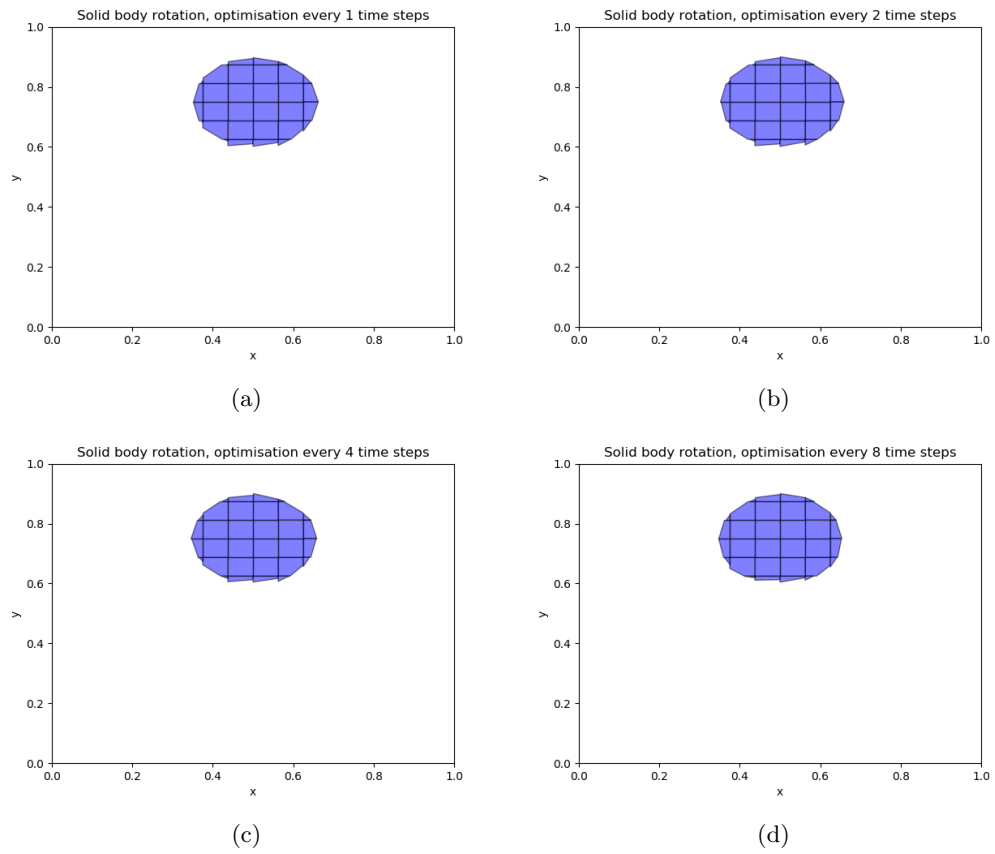
Figure 25: Volume of fluid fields when taking more time steps per optimisation routine for solid body rotation, table 2.
