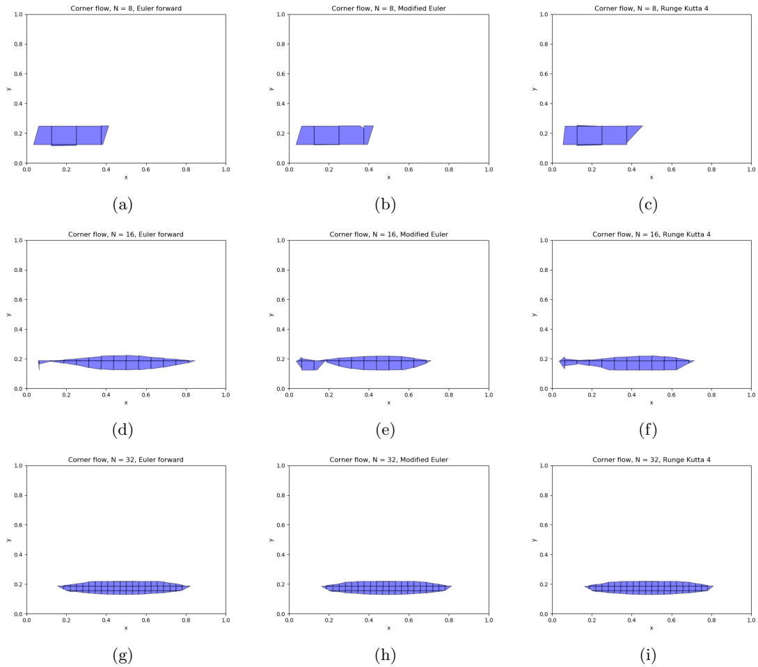
Figure 21: Volume of fluid fields for the test of table 1 for the corner flow test. The velocity field is handled much better than the solid body rotation test and no obvious instabilities are visible.
