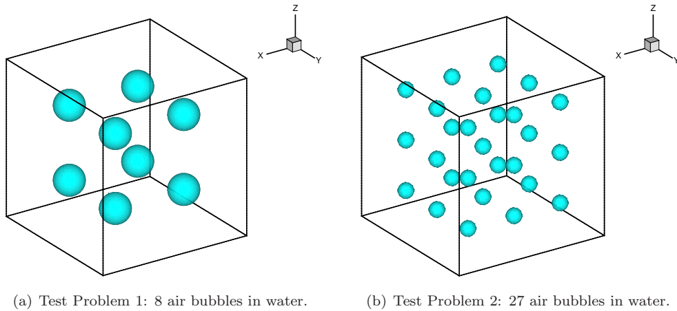
Figure 1: Geometry of bubbly flow test problems.
