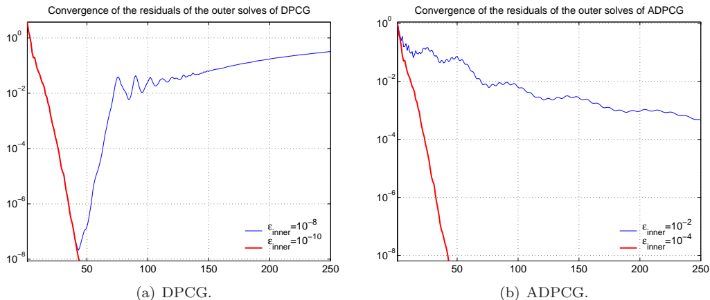
Figure 3: Convergence of the residuals of the outer iterations from DPCG and ADPCG with k = 25^3 (Test Problem 2).
